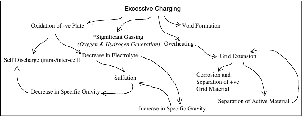
Figure 2-5 Failure modes associated with inadequate battery charging.
